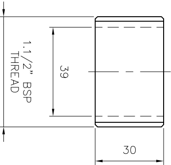
(SCALE-1:4) DETAIL-A BUSH FOR COUPLER
